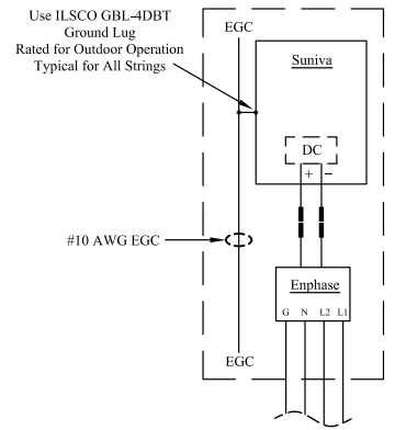
Typical Microinverter and Module Wiring Configuration, (1) Inverter Per Module
